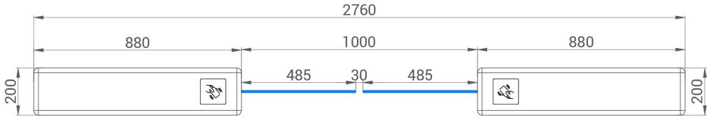
Top View
